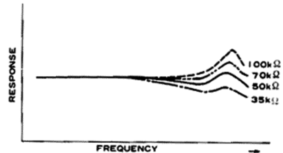
Cartridge frequency response graph according to impedance setting.
