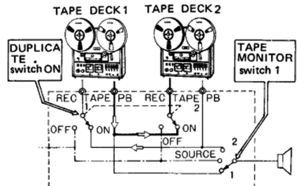
Duplication: Playback signal from tape deck 1 in the figure enters via TAPE 1 PB jacks, passes through DUPLICATE switch ON, and is recorded by tape deck 2. This can also be performed in reverse, ie: playback with tape deck 2 and record with tape deck 1.
