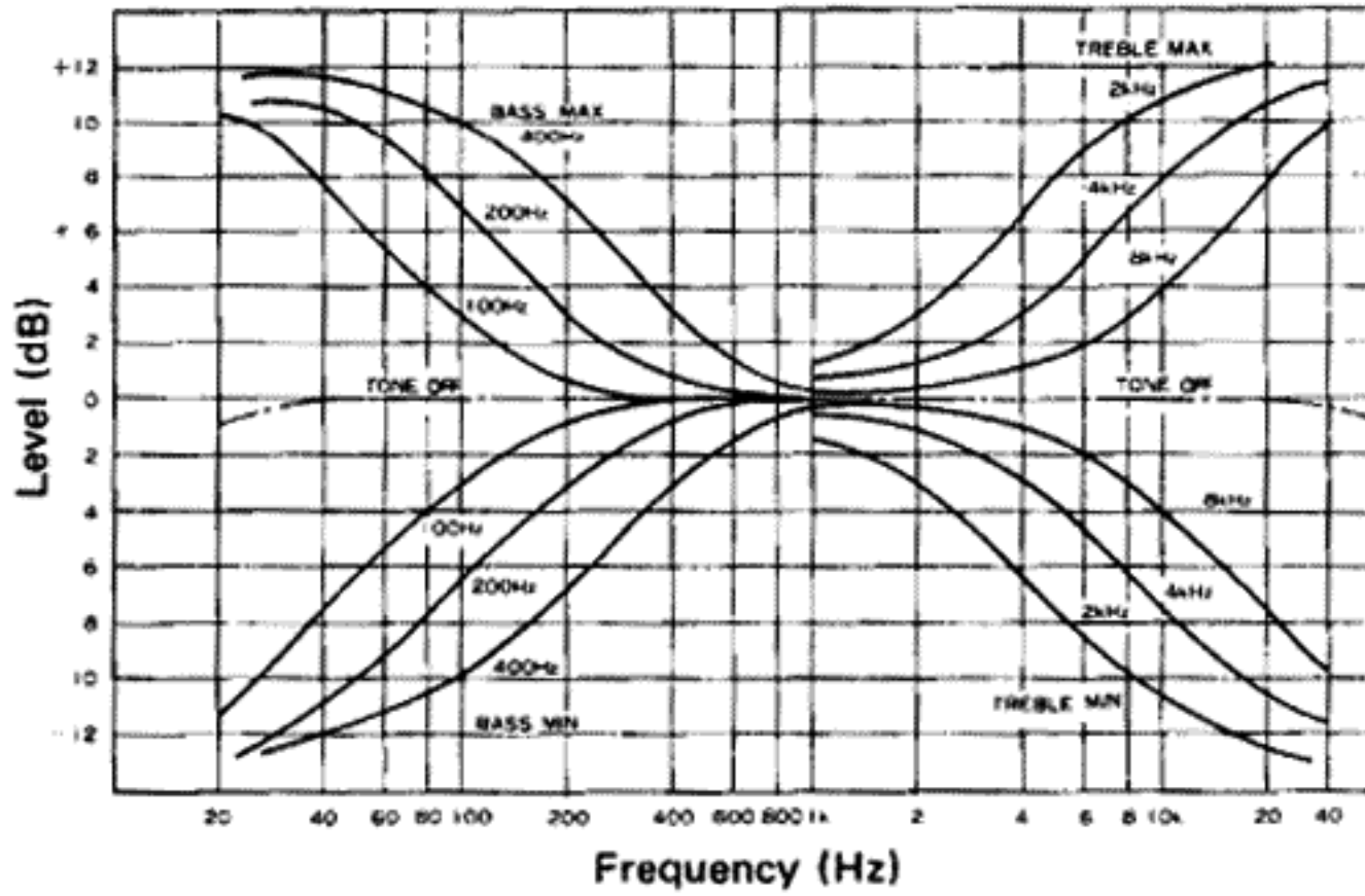
RESPONSE GRAPH
